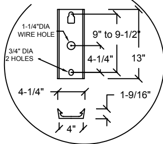
DETAIL OF MOUNTING PLATE
